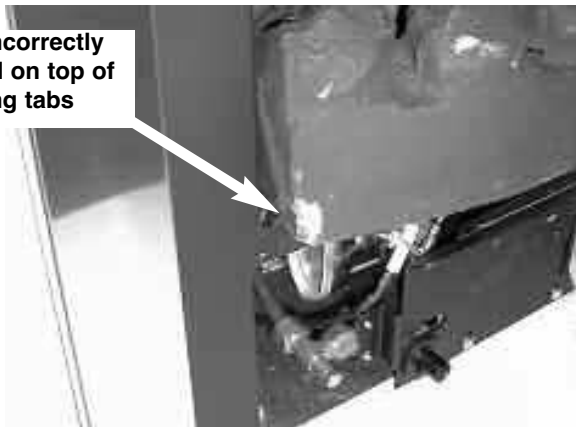
Fig. 26b - Shows incorrect location of fuelbed
